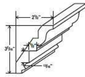
Angle Light Rail Moulding
