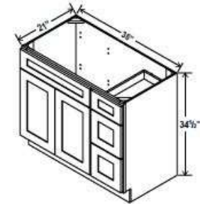
V3621DL: 36" combo with drawers on left V3621DR: 36" combo with drawers on right
