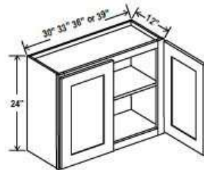
One adjustable shelf
